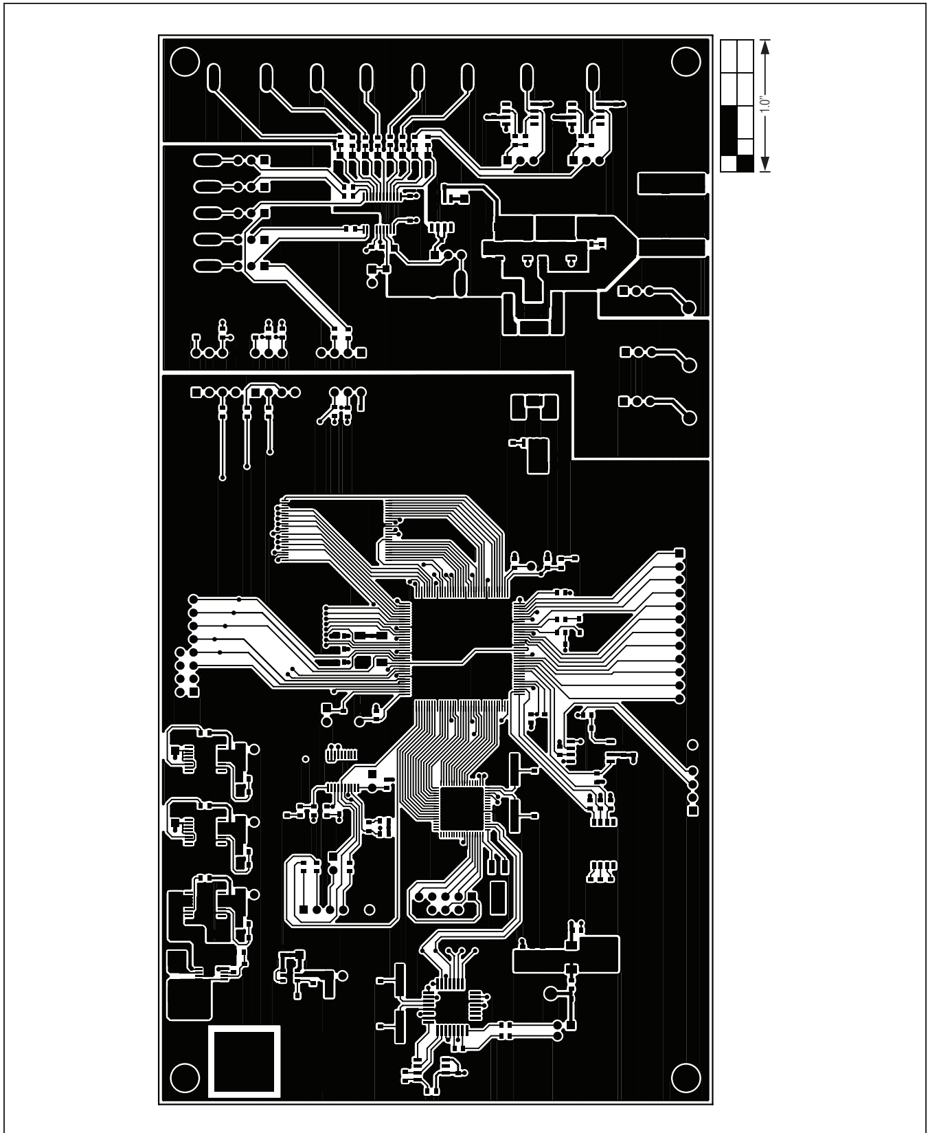
Figure 9. MAX1300A EV Kit PCB Layout—Component Side
