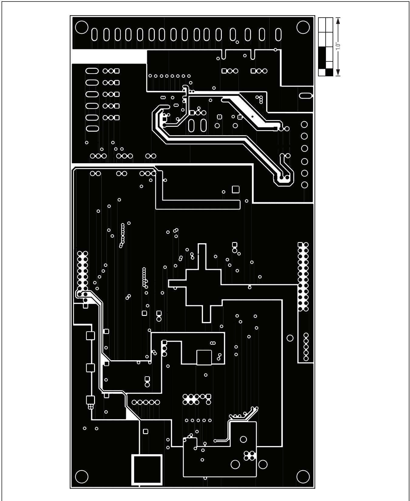
Figure 11. MAX1300A EV Kit PCB Layout—Layer 3
