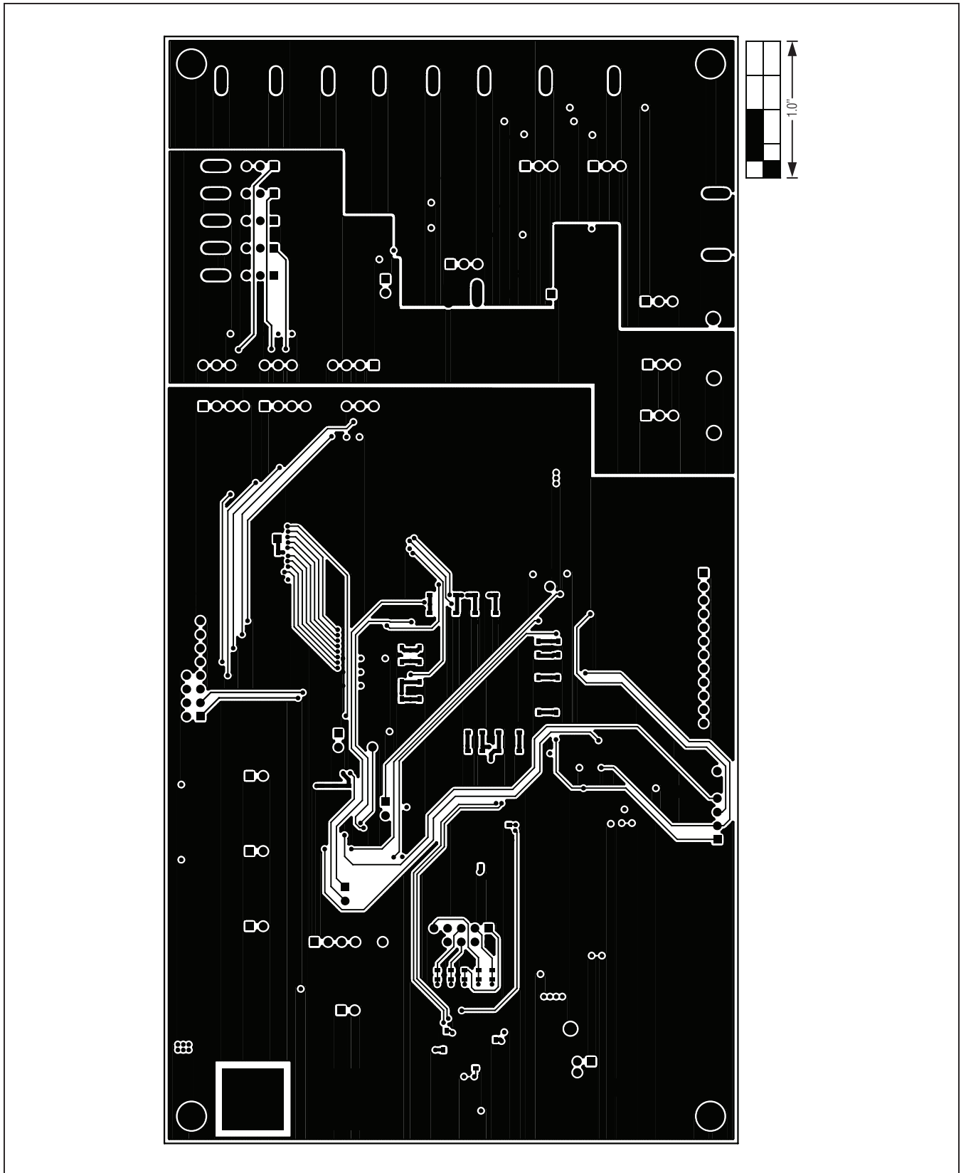
Figure 12. MAX1300A EV Kit PCB Layout—Solder Side
